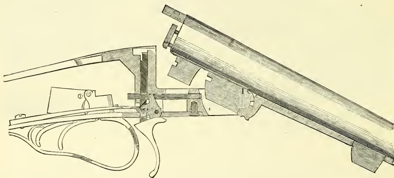
The Abbey Breech-loader.
